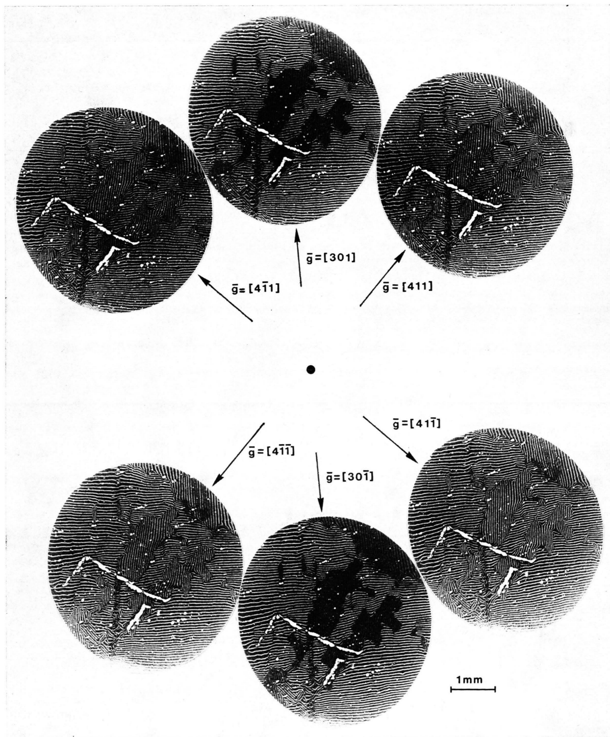
Fig. 2. A Laue pattern of six enlarged back-reflection topographs from an iron-3% silicon crystal taken with synchrotron radiation from the DORIS storage ring simultaneously on one film. Altogether 15 pairs of topographs may be viewed stereoscopically from suitable directions. The accelerator conditions were 3.3 GeV, 40 mA; exposure time 60 s.
